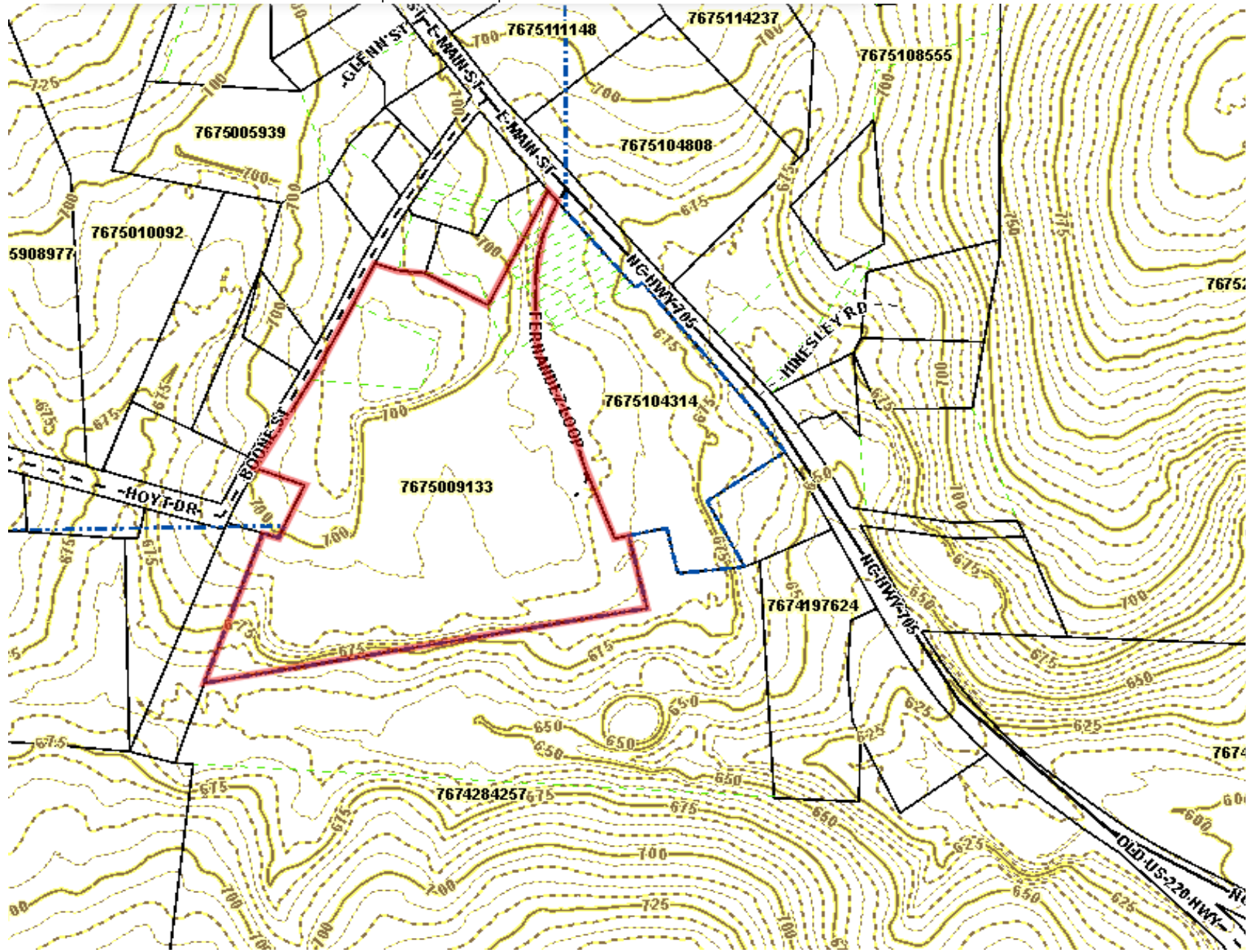
Sapona Plastics Plant 2 - Storm Water Pollution Prevention - site plan contour map
